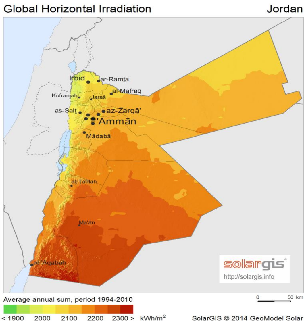
Figure ( ): Global Horizontal Insulation in Jordan 34
