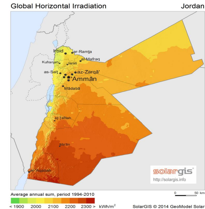
Annual Global Horizontal Insolation in Jordan 38
