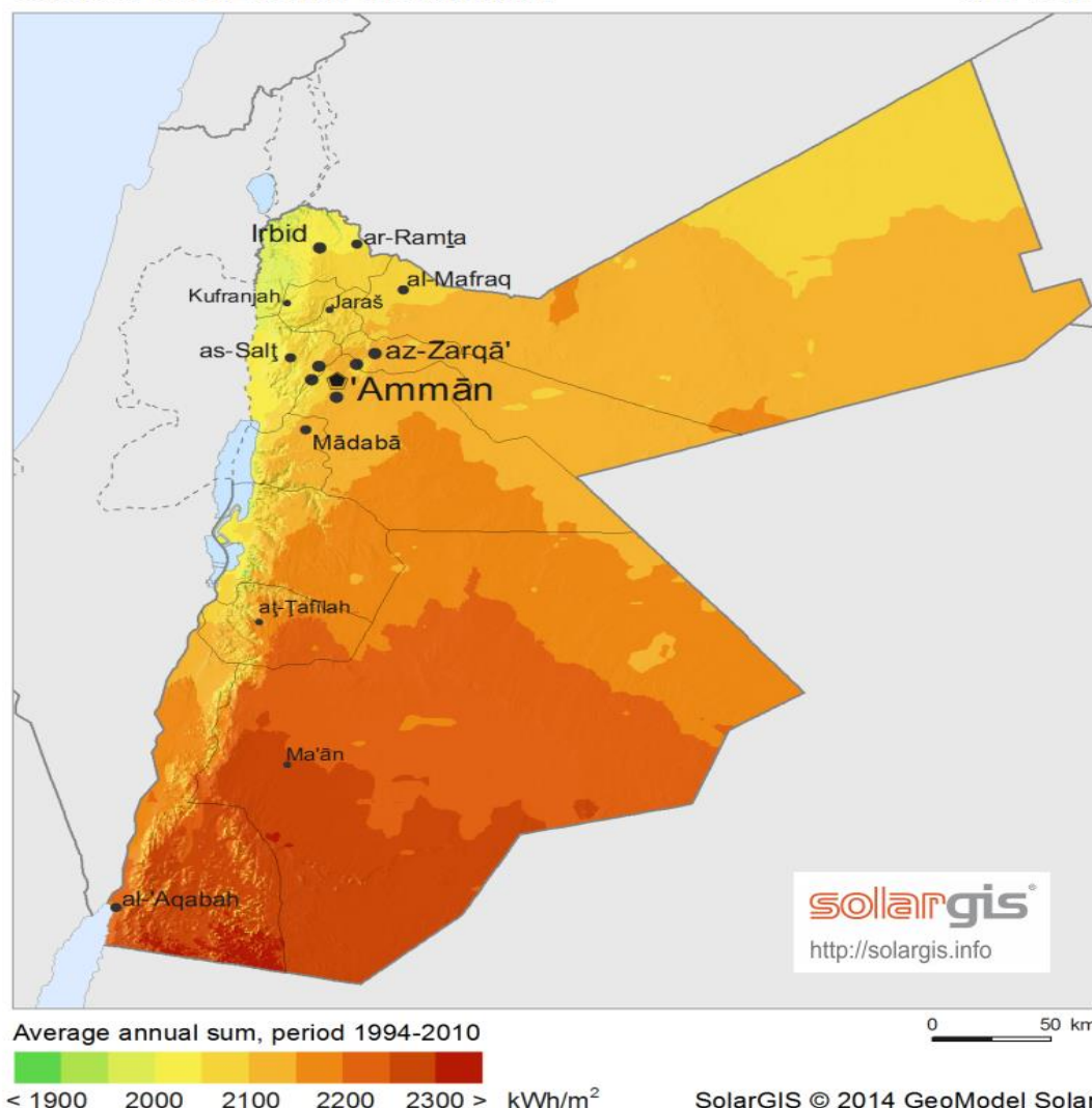
Figure ( ): Global Horizontal Insulation in Jordan 36
